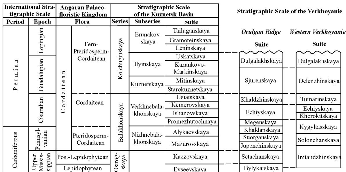
Figure 1. Correlation of Palaeozoic stratigraphic schemes of Verkhoyanie and Kuznetsk Basin
